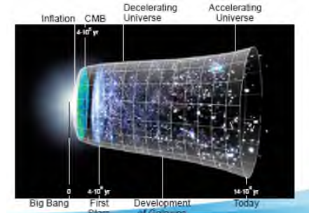
EUCLID objective: to study geometry and nature of the dark universe
