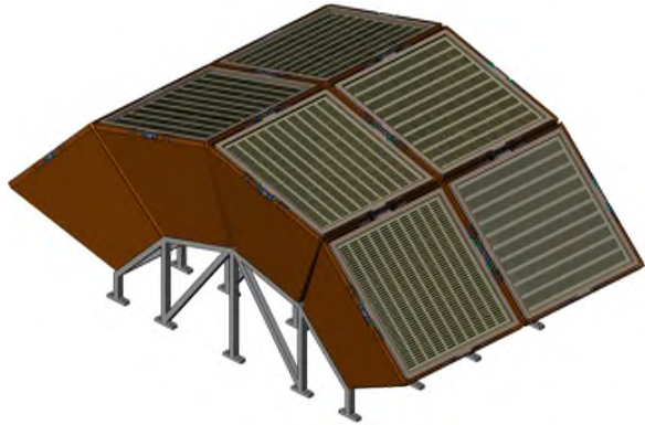
LOFT/ WFM Collimator, Mask & Detector Tray
