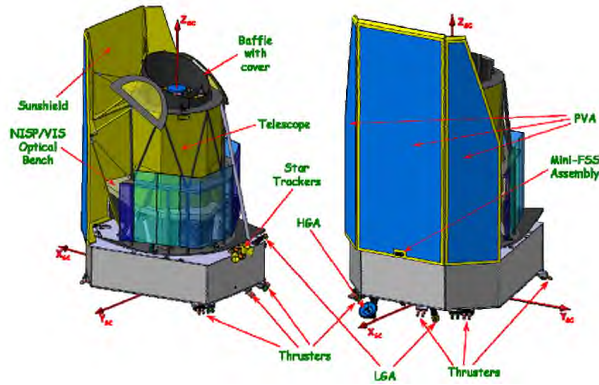
EUCLID Satellite and Payload
