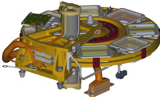
Filter Wheel for NAC Camera (Rosetta satellite)
