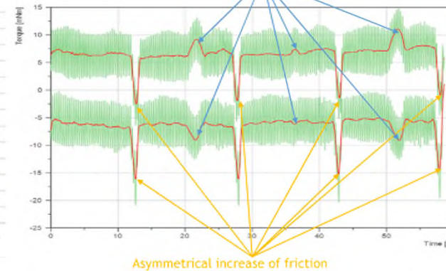
Friction variation due to contact between smile of cross
