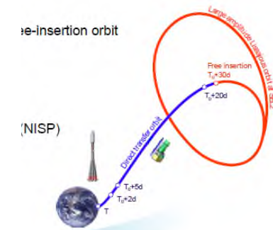
L2 Lagrangian point orbit
