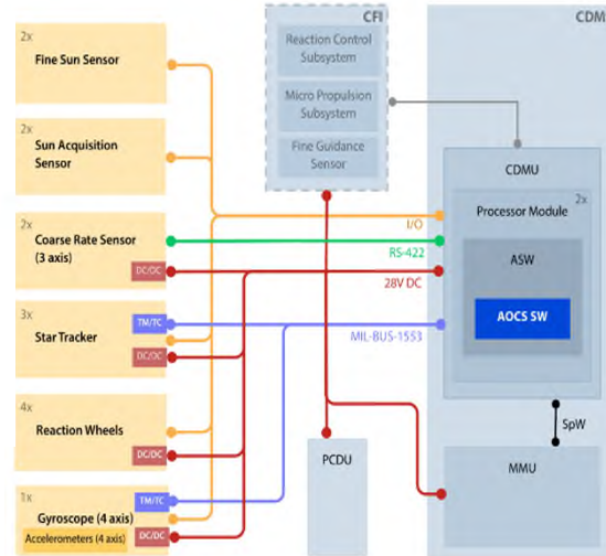
High accuracy AOCs
