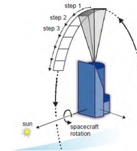
Step and stare observation mode
